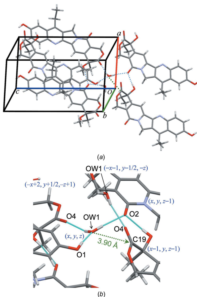
Figure 3 (a) The crystal packing of SN-38 monohydrate. Hydrogen bonds are shown as blue dotted lines. The O atom of the water molecule and a carbonyl C atom in the lactone ring nearest to the water molecule are connected with a green dotted line. (b) The hydrogen-bond network around the water molecule.
