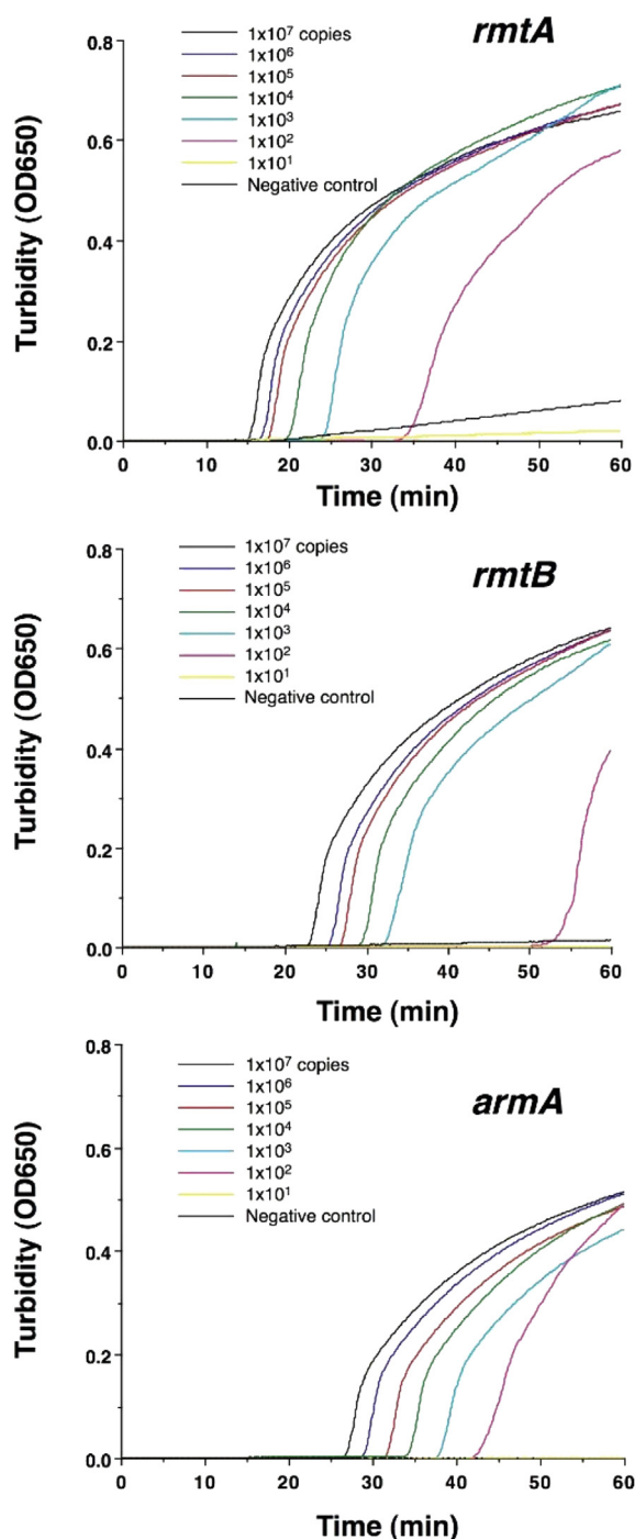
Fig. 1. Detection sensitivity and reaction time of the LAMP assays for rmtA , rmtB , and armA . Turbidity was monitored by a Loopamp real-time turbidimeter LA-320 at 650 nm.
