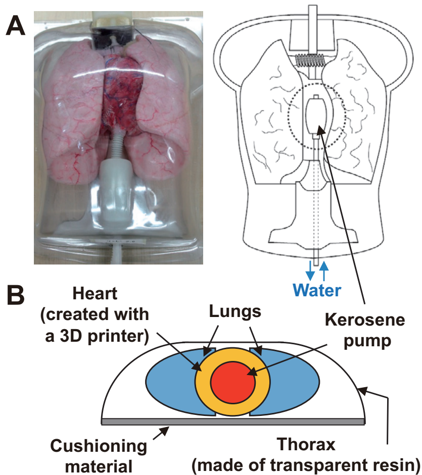
Fig. 2 External view (A) and structure (B) of prototype. A simulated heart is embedded in the chest of a mannequin of the upper half of a human body. Its forward-facing portion where the chest is present has a shape simulating the human body, while its backward-facing portion is a flat plate. In addition, simulated lungs are disposed on both sides of simulated heart.
