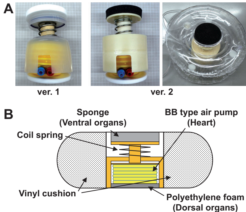
Fig. 3 External view (A) and structure (B) of “Dock-kun ver. 1” (ver. 1) and “Dock-kun ver. 2” (ver. 2). The air pump was housed in a cylinder, and the coil spring and upper and lower cushioning materials were used in both ver. 1 and ver. 2. The differences of structure between ver. 1 and ver. 2 include the type of air pump, the material and thickness of the cushioning materials, and the rigidity of the cylinder. Thus, the optimal amount of water to simulate blood could be better pumped out only when correct chest compression and decompression were performed with ver. 2 in comparison with ver. 1.
