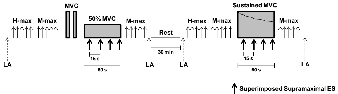
Figure 1. A schematic presentation of the protocols performed in Experiment I. The upper diagram represents the 15 second ramp to MVC and the bottom diagram represents the 60 second sustained 50% MVC and the 60 second sustained MVC. Arrows represent electrical stimuli to evoke maximal resting H-reflexes, M responses and twitch force. The bold arrows represent superimposed supramaximal electrical stimuli (ES) to evoke corticospinal (M and V responses) and superimposed twitch responses and the dotted arrows represent blood lactate (LA) measurements.
