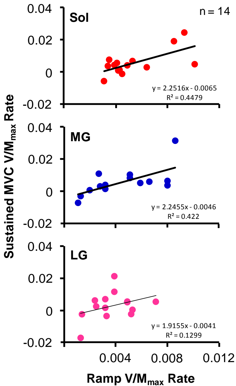
Figure 12. Relationship between the rate of increase in V response amplitude during the 15 second ramp to MVC and the rate of decrease/increase in V response amplitude during the 60 second sustained MVC. A significant relationship was observed in Sol ( r = 0.669 , p < 0.01 ) and MG ( r = 0.650 , p < 0.05 ). No relationship was observed in LG.
