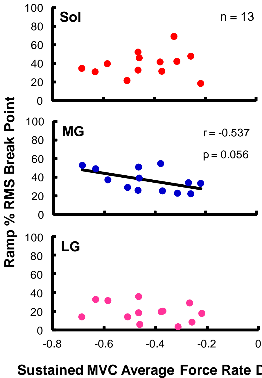
Figure 10. Relationship between 60 second sustained MVC force rate decline and 15 second ramp to MVC rmsEMG BPs in 13 subjects for each muscle. A trend toward significance was observed in only the MG ( r = -0.537 ; p = 0.056 ).
