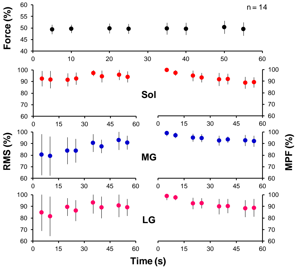
Figure 16. Normalised force (upper panel), rmsEMG (left panel) and MPF (right panel) of Sol, MG and LG during the 60 second sustained 50% MVC in 14 subjects. A significant increase in rmsEMG was observed in Sol ( r = 0.664 ), MG ( r = 0.937 ) and LG ( r = 0.695 ) and a significant decrease in MPF was observed in Sol ( r = 0.973 ), MG ( r = 0.933 ) and LG ( r = 0.948 ). All data are mean \pm SD.
