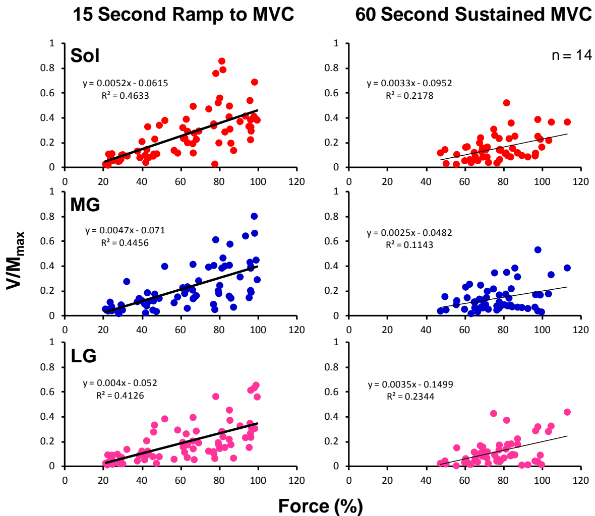
Figure 11. Relationship between normalised force (%MVC) and normalised V response amplitude ( V/M_{max} ) during the 15 second ramp to MVC (left panel) and the 60 second sustained MVC (right panel). A significant increase in V response amplitude was observed in Sol ( r = 0.681 ), MG ( r = 0.668 ) and LG ( r = 0.642 ) during ramp and a trend toward a significant decrease in V response amplitude was observed in Sol, MG and LG during sustained MVC.
