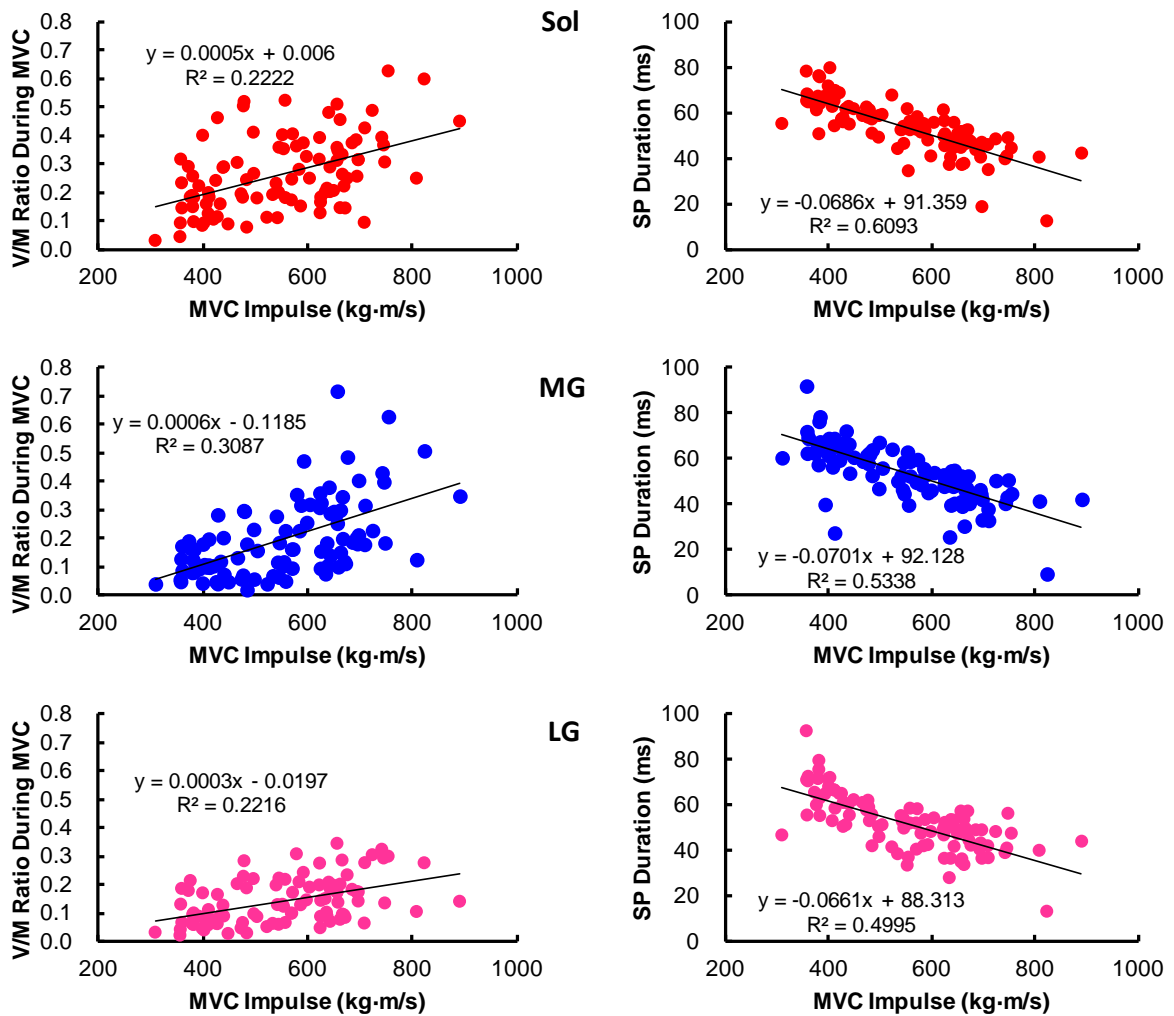
Figure 20. Relationship between impulse and V/M ratio (left side), and silent period duration (right side) during intermittent MVCs. Significance ( p < 0.01 ).
